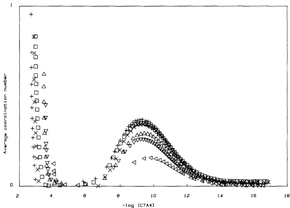
Fig. 1. Experimental formation curve for the magnesium-citrate system (NDP = 4 for citrate). The following symbols +, X, □, △, ▽, ◁, correspond to the respective order of experiments summarized in Table I.
