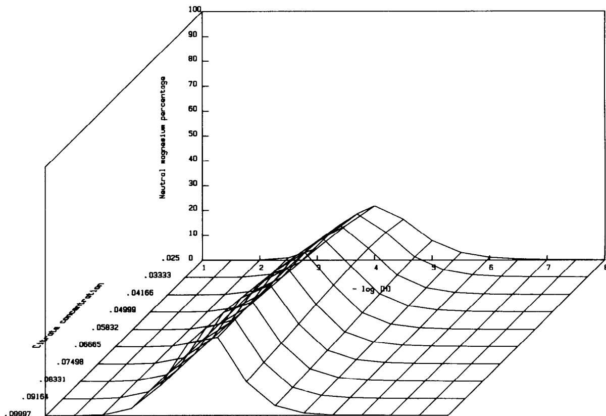
Fig. 5. Distribution of the neutral fraction of magnesium in the presence of different concentrations of citrate ( C_{Mg} = 0.025 \text{ mol dm}^{-3} ).
