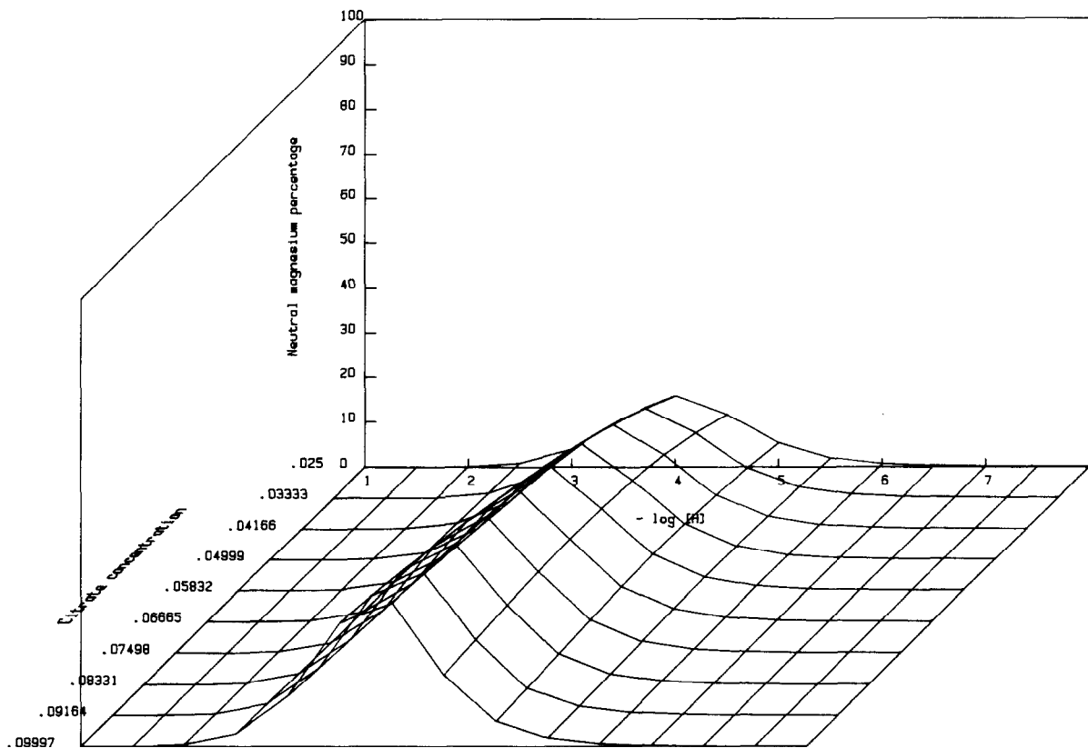
Fig. 6. Distribution of the neutral fraction of magnesium in the presence of 0.025 \text{ mol dm}^{-3} of calcium and of different concentrations of citrate. Magnesium concentration is the same as in Fig. 5.
